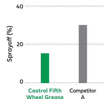
ASTM D4049 Water Sprayoff Test
