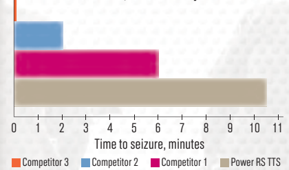
Castrol High Speed Lubricity Test 8000 rpm, 260°C, 400:1 fuel/oil
