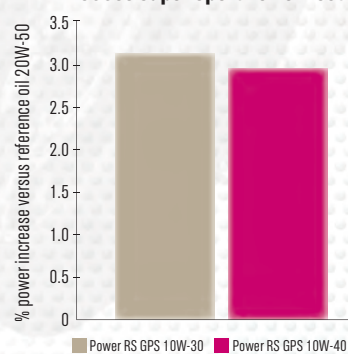
600cc Super Sport Power Test
