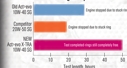
Castrol High Temperature Test
