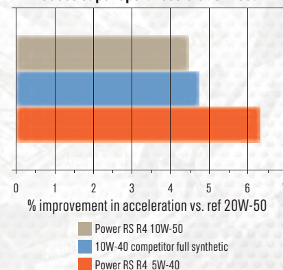
600cc Super Sport Acceleration Test
